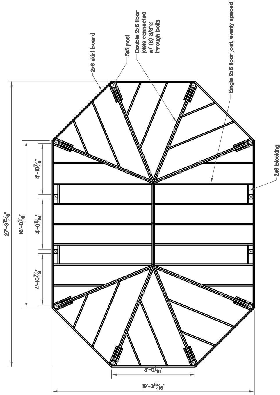
Floor Plan 20'x28'
